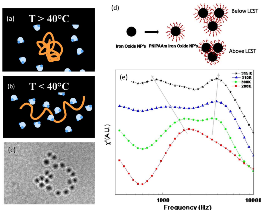
Fig. 15. A typical temperature sensitive polymer, p-NIPAAm shows a conformational change at a critical temperature, LCST. For example, (a) at T > \text{LCST} ( = 40^\circ\text{C} ) the polymer is collapsed but (b) is open at T < \text{LCST} . (c) p-NIPAAm functionalized magnetite nanoparticles. (d) Pictorial representation of the behavior of p-NIPAAm functionalized magnetite nanoparticles below and above LCST. Note that when the p-NIPAAm collapses for T > \text{LCST} the nanoparticles become less hydrophilic and agglomerate. (e) The physical change in size can be monitored by ac susceptibility measurements. The peak at higher frequency shifts to larger values with increasing temperature corresponding to the shrinking of the nanoparticle V_H ; however, the particles now become hydrophobic and then agglomerate as reflected in the emerging peak at lower frequencies.
